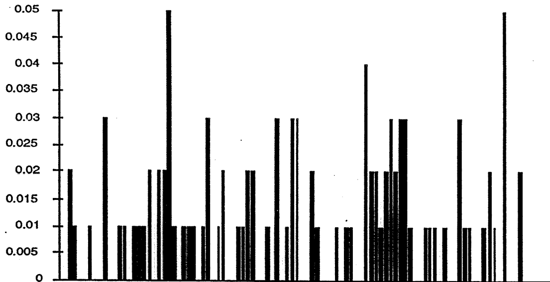
Hundred trials
