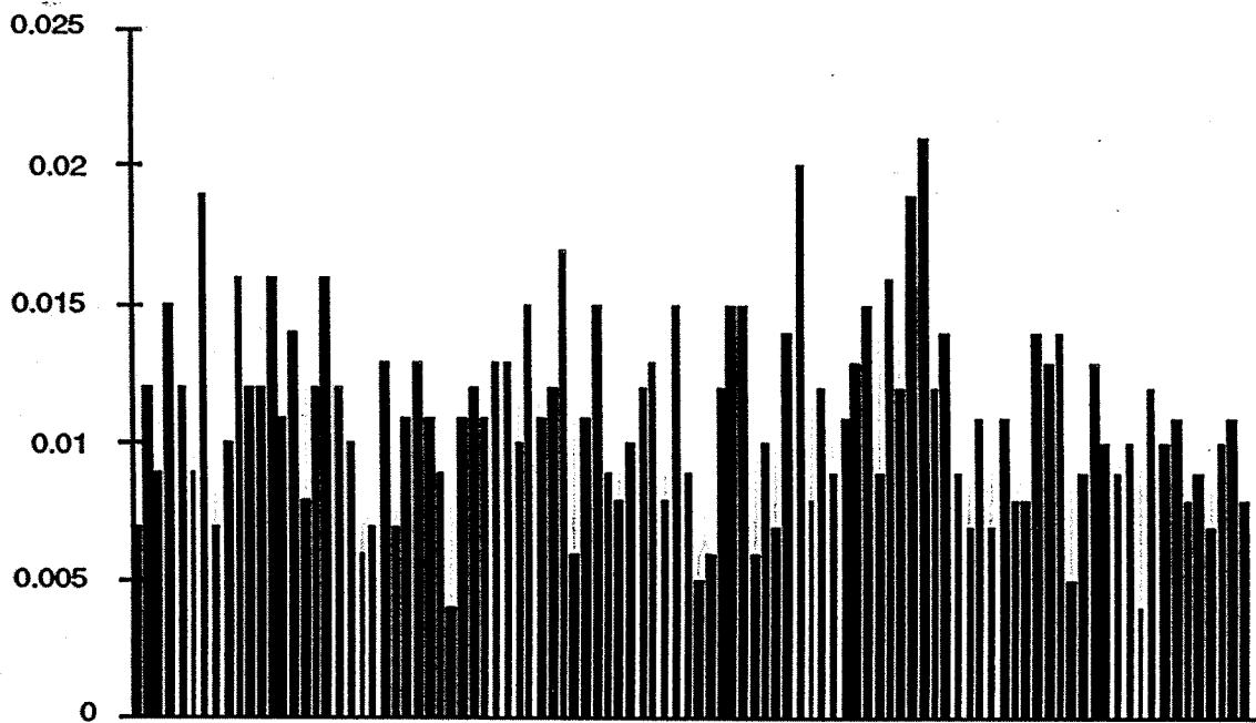
Thousand trials
